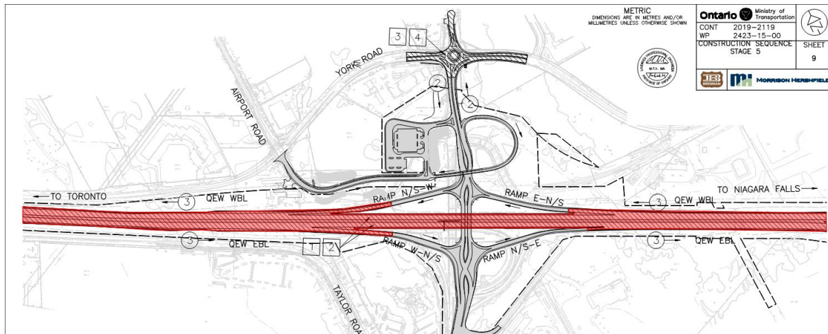
Figure 1: Approximate Work Area on QEW within QEW/Glendale Interchange
