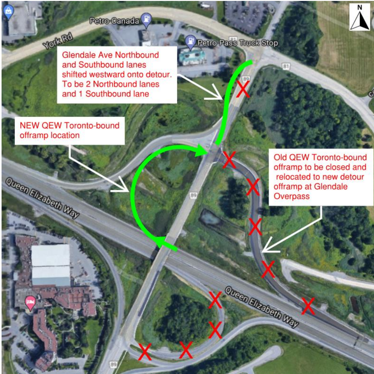
Figure 1: Stage 3 traffic changes shown by green detour lines. Closed roadways/ramps shown by Red X's.
