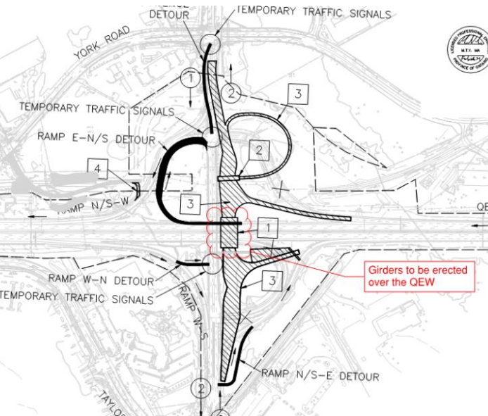
Figure 1: Plan Location for Precast Concrete Girder Erection and Typical Crane Erection
